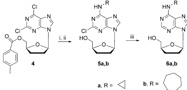
Scheme 2. Synthesis of (2-chloro)-6-cycloalkylamino-9-(2,3-dideoxy- \beta - D -glyceropentofuranosyl)-9H-purines: (i) R-NH 2 ; (ii) NH 3 /CH 3 OH; (iii) Pd/C, H 2 , OH - .
