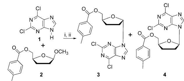
Scheme 1. Synthesis of 2,6-dichloro-9-(2,3-dideoxy- \alpha -D-glycero-pentofuranosyl)-9H-purine and 2,6-dichloro-9-(2,3-dideoxy- \beta -D-glycero-pentofuranosyl)-9H-purine: (i) HMDS, (NH 4 ) 2 SO 4 , \Delta ; (ii) CH 3 CN, TMSTf.
