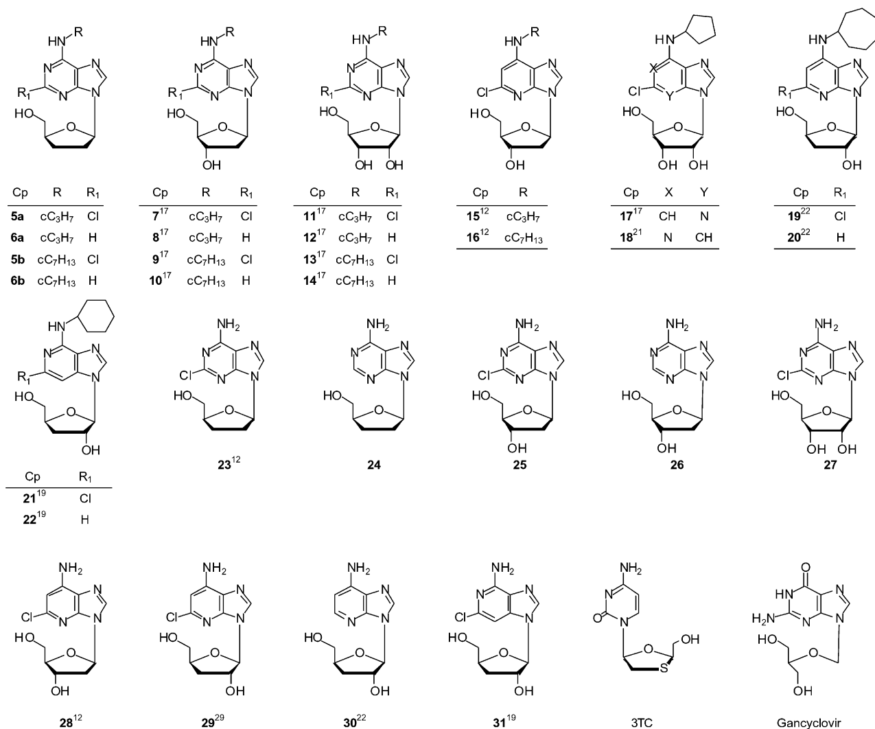
Figure 1. Structure of tested compounds. 21–23
